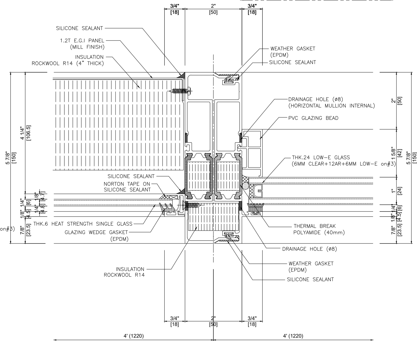
"A" DETAIL (scale : 2/1) : Heel bead dimension reference
