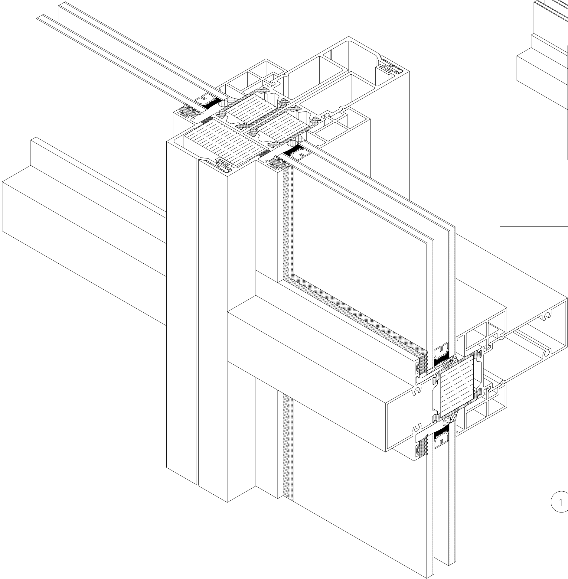
Mechanical joint (hor-to-vert)
