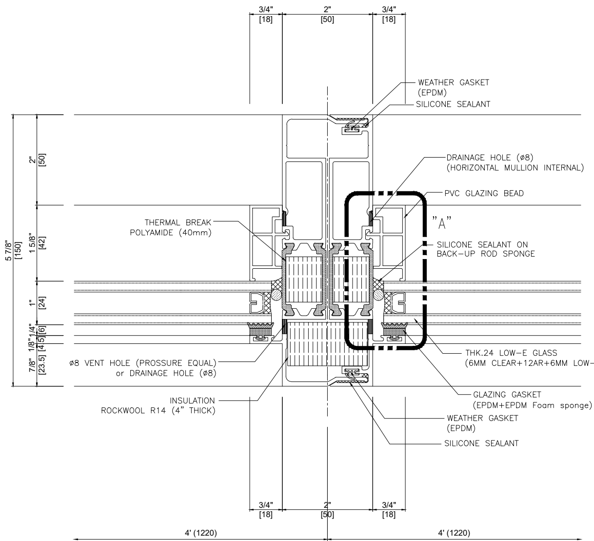
1 HORIZONTAL SECTION
