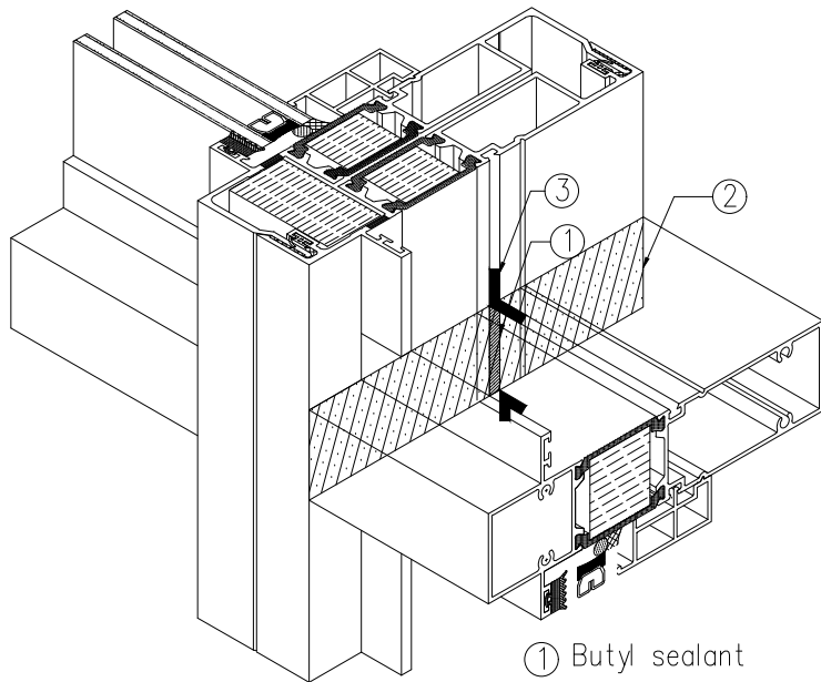
Mechanical joint (hor-to-vert)
